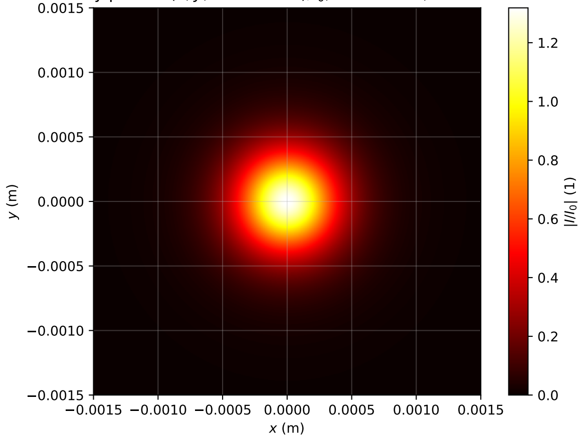
Intensity profile I(x, y, z = 1.990m)/I_0 , P_{in}=0.8P_{cr} , artificial time
